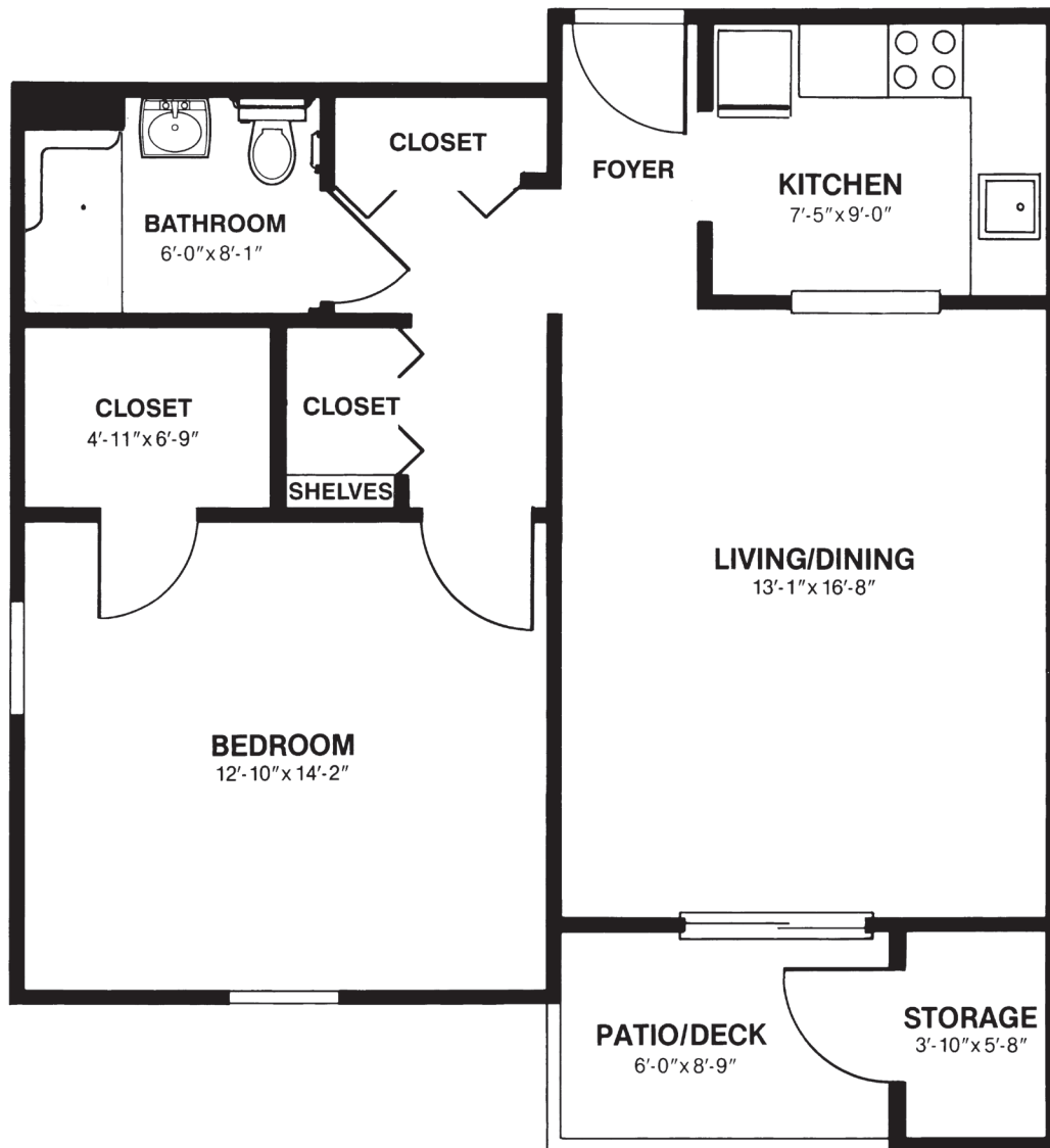
Corner 1 Bedroom, 1 Bath 672 Square Feet
